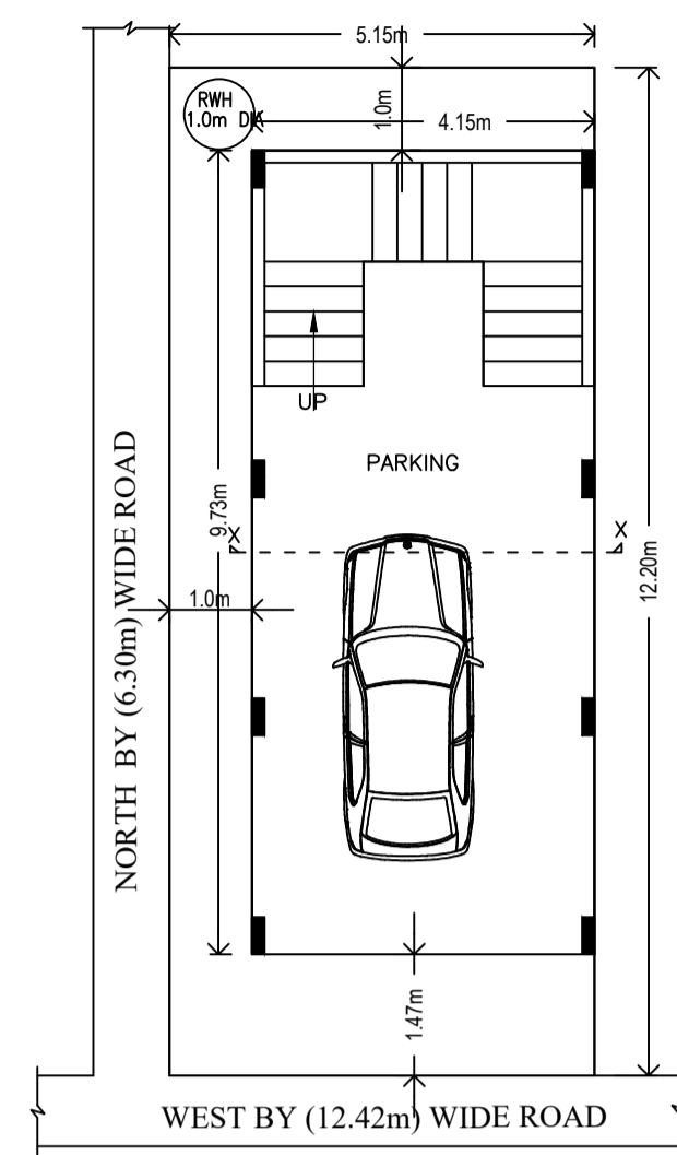
STILT FLOOR PLAN
