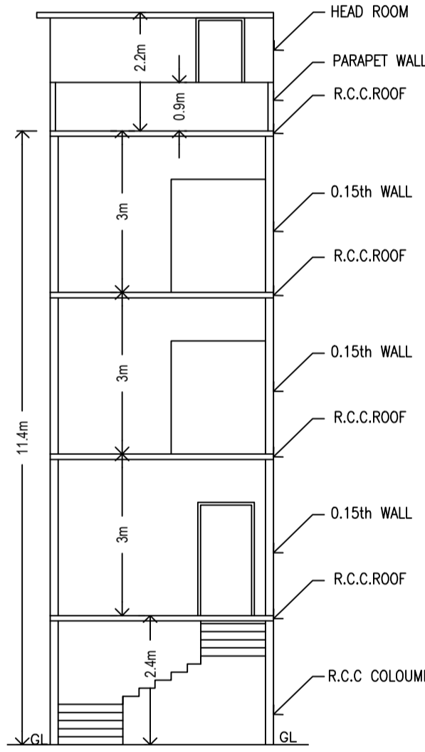
SECTION @ X-X
